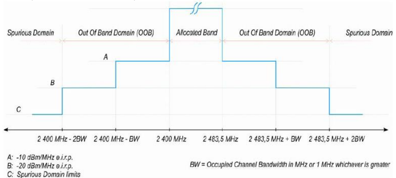
Figure 3: Transmit mask
