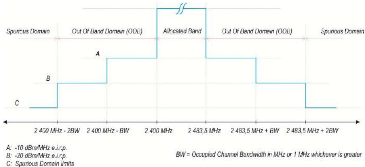
Figure 1: Transmit mask
