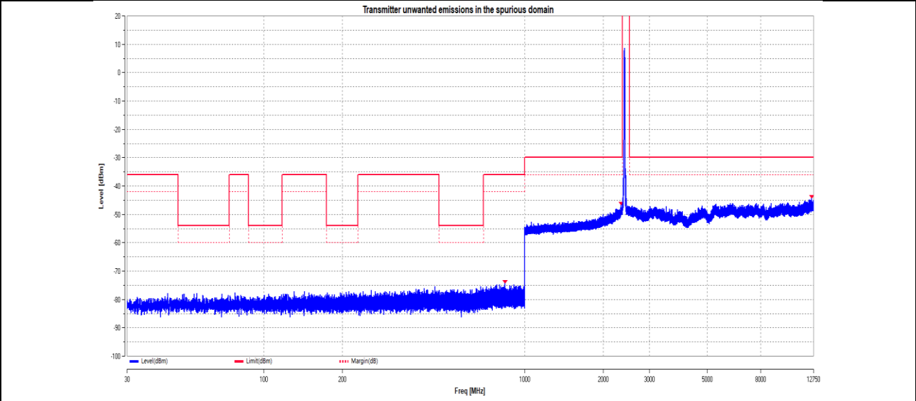
11G Ant2 2412
