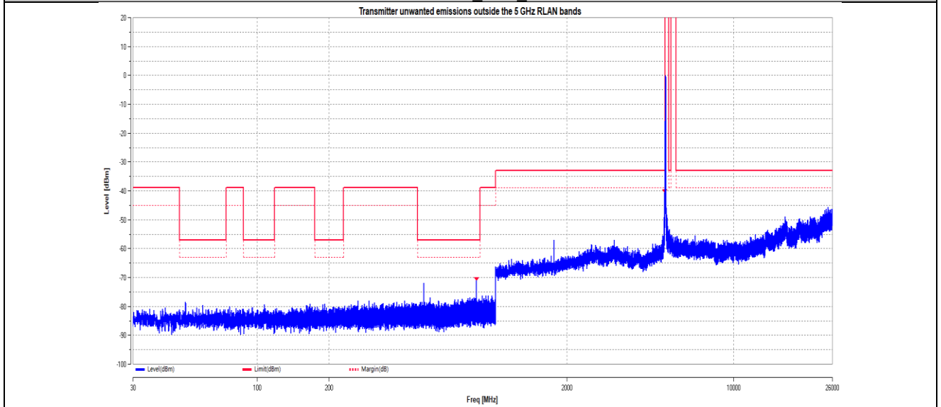
11N40MIMO Ant2 5190
