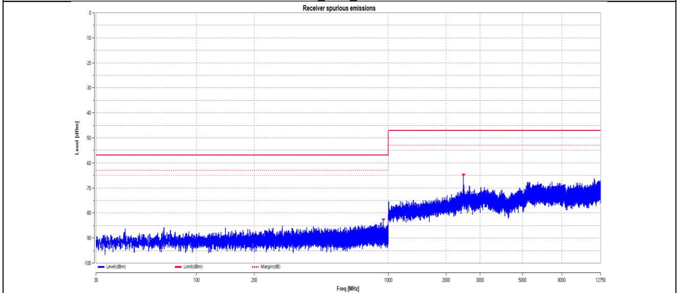
11G Ant2 2412
