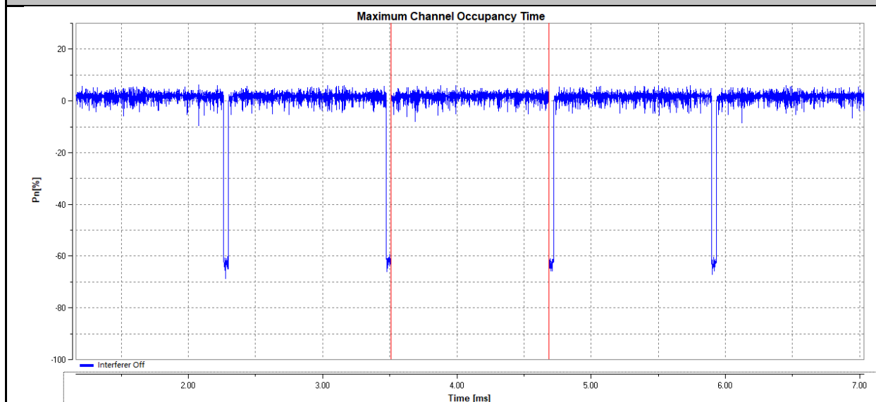
Adaptivity_Max.COT_TNVN_11A_5180_Ant1
