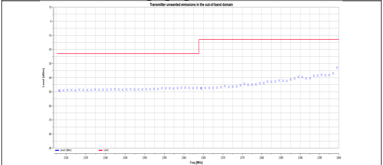
11N40MIMO Ant1 2422 2483.5MHz+2BW
