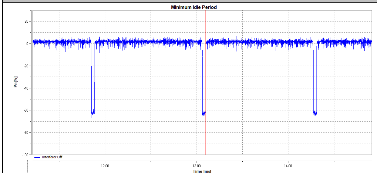
Adaptivity_Min.IdleTime_TNVN_11A_5180_Ant1
