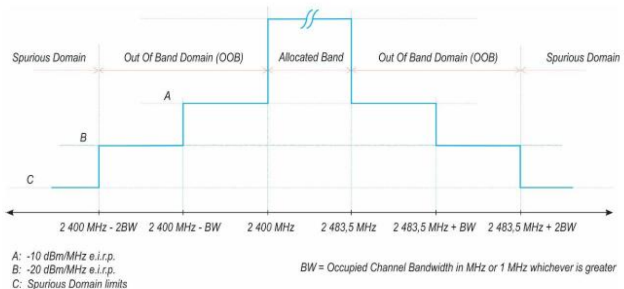
Figure 3: Transmit mask
