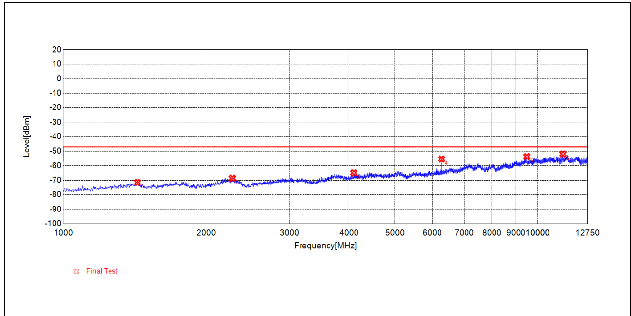
(RX_RSE_BLE_2Mbps_2480MHz_1GHz to 12.75GHz_Antenna Vertical)
