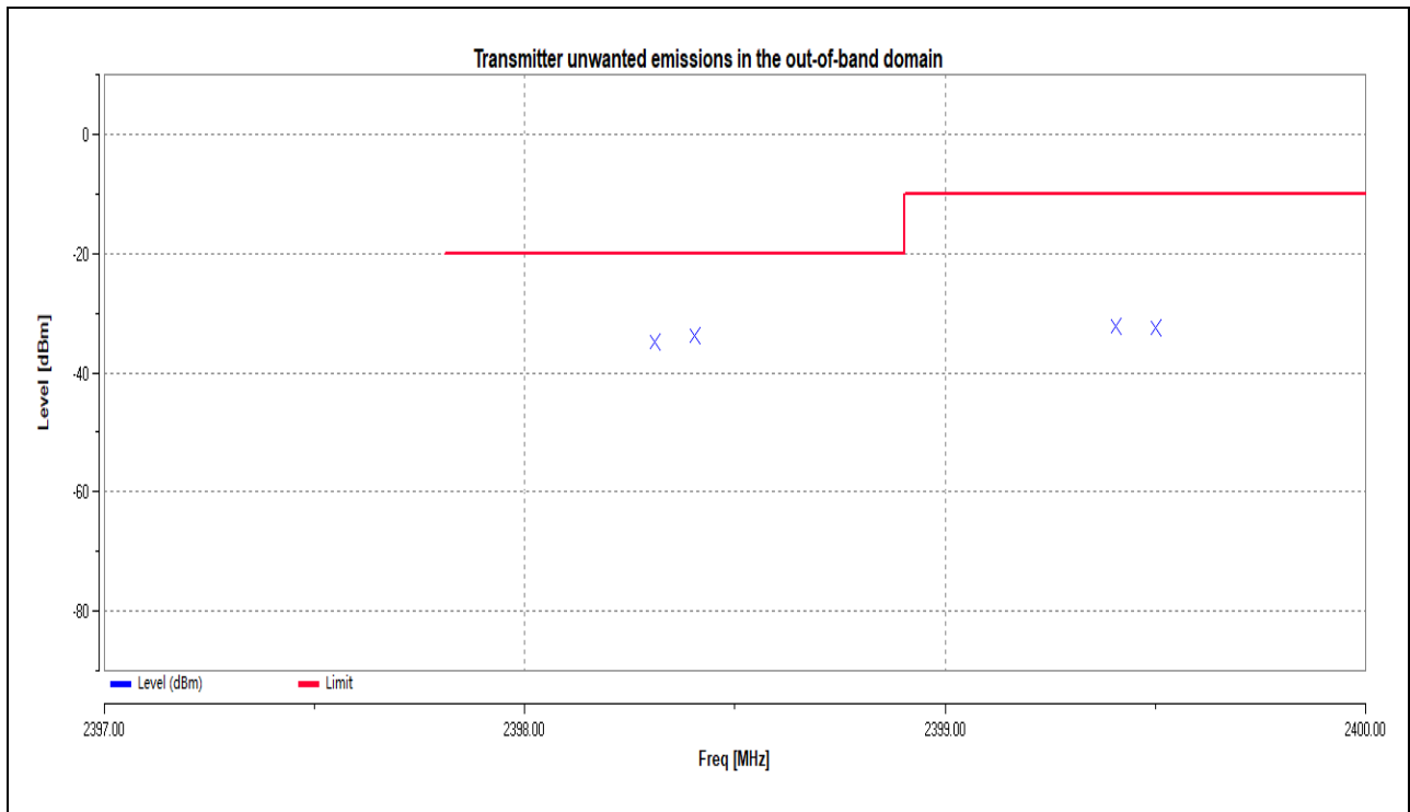
(OOB_BLE_1Mbps_2402MHz)
