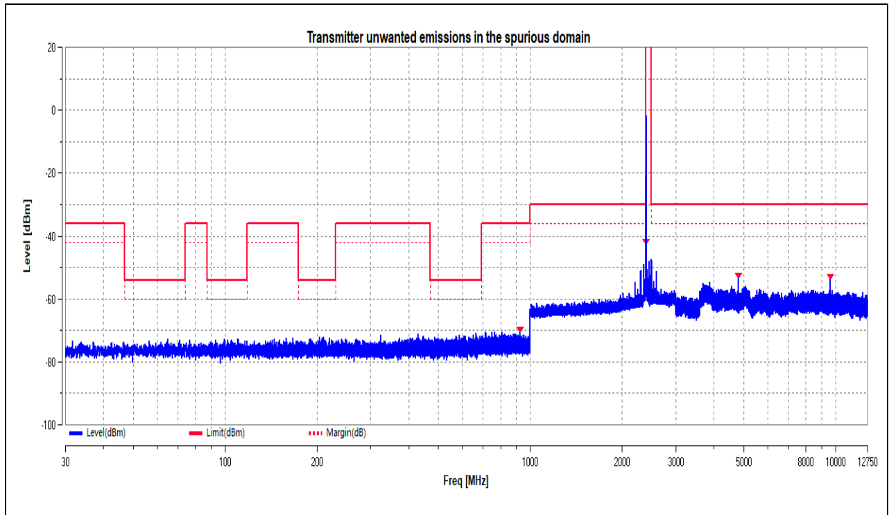
(TX_CSE_BLE_2Mbps_2402MHz_30MHz to 12.75GHz)
