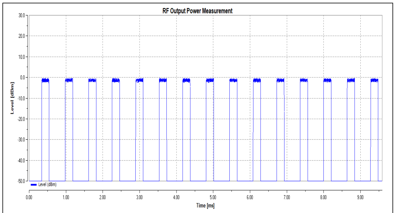
(Output Power_ BLE_2Mbps_2440MHz)
