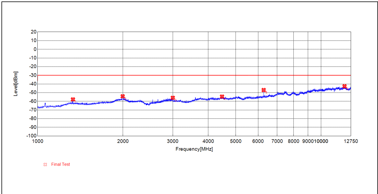
(TX_RSE_BLE_1Mbps_2402MHz_1GHz to 12.75GHz_ Antenna Horizontal)
