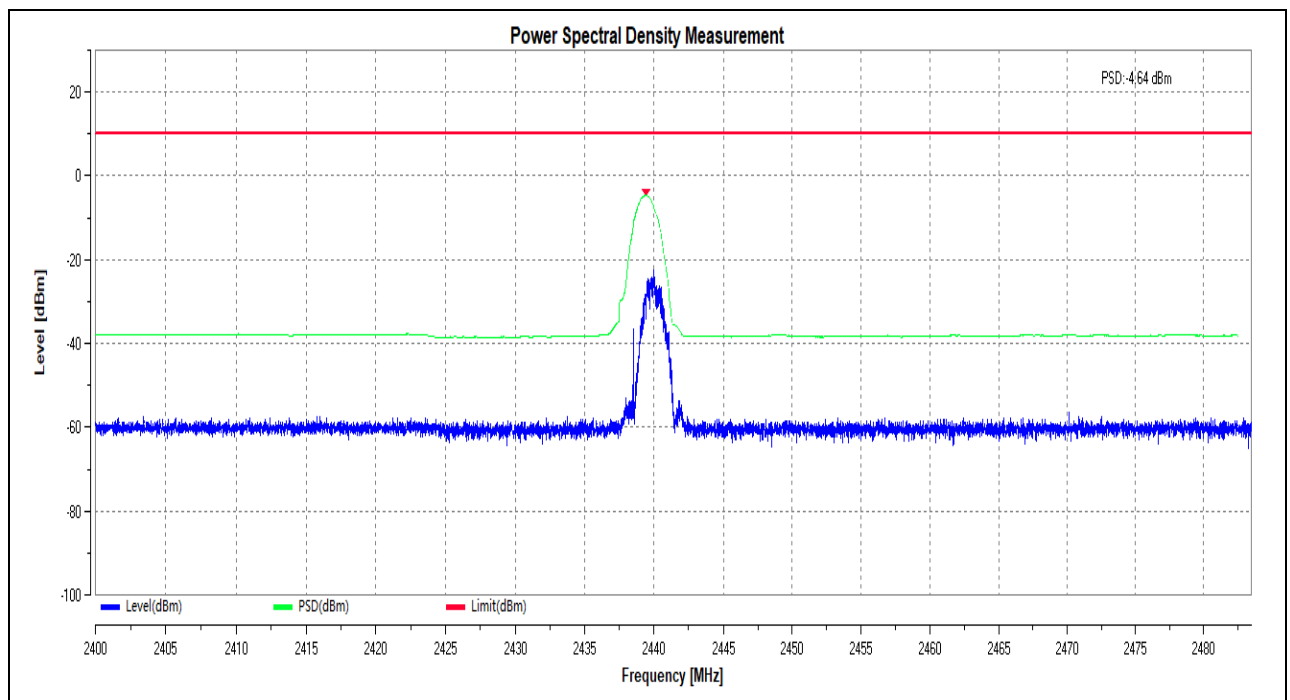
(Power Spectral Density _BLE_2Mbps_2440MHz)
