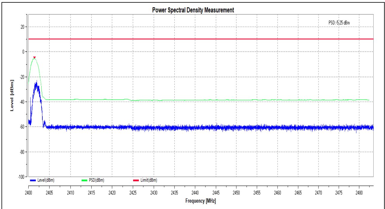
(Power Spectral Density _BLE_2Mbps_2402MHz)
