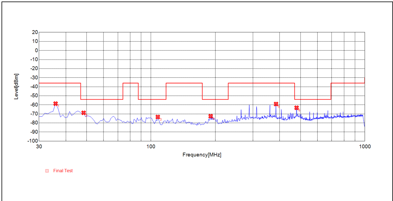
(TX_RSE_BLE_2Mbps_2402MHz_30MHz to 1GHz_Antenna Vertical)
