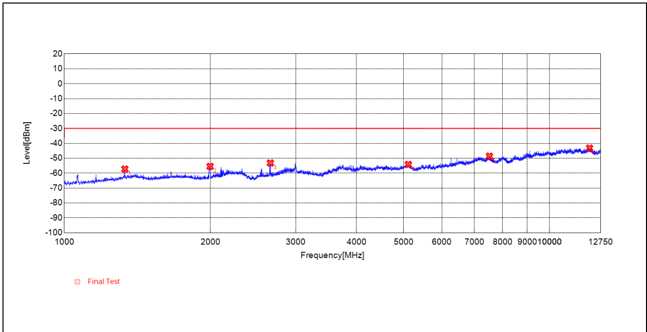
(TX_RSE_BLE_2Mbps_2402MHz_1GHz to 12.75GHz_Antenna Vertical)
