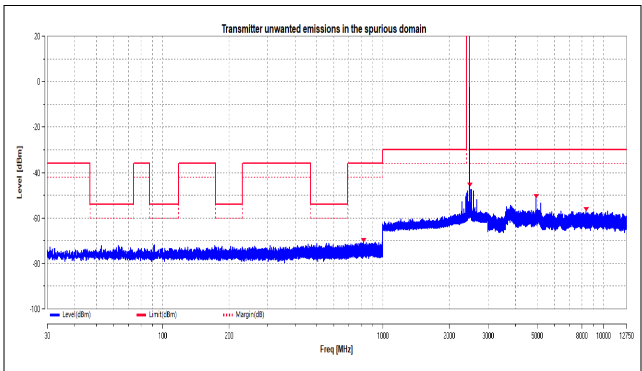
(TX_CSE_BLE_1Mbps_2480MHz_30MHz to 12.75GHz)
