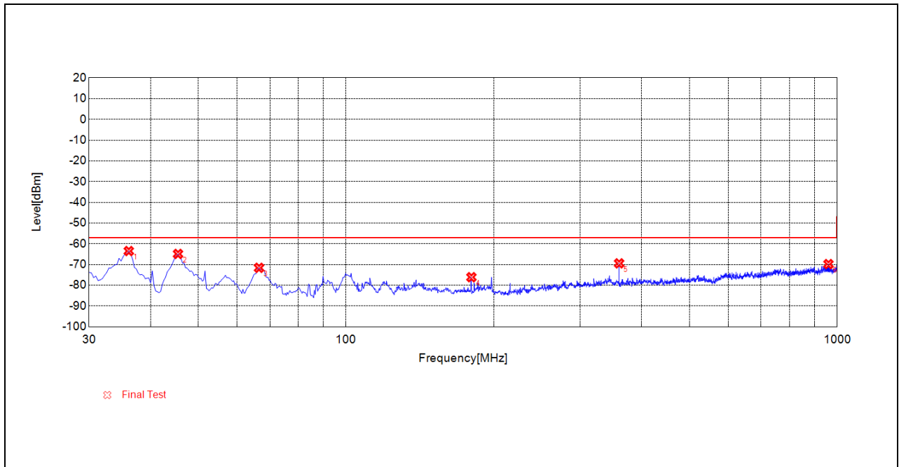
(RX_RSE_BLE_1Mbps_2402MHz_30MHz to 1GHz_Antenna Vertical)
