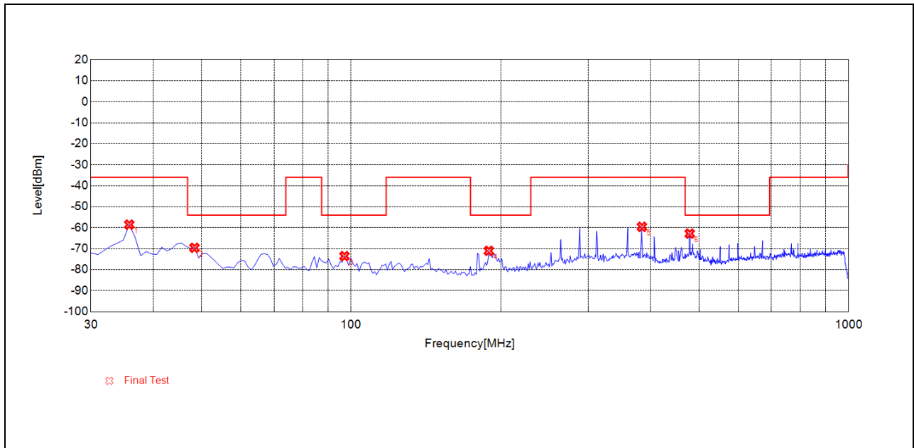
(TX_RSE_BLE_1Mbps_2480MHz_30MHz to 1GHz_Antenna Vertical)
