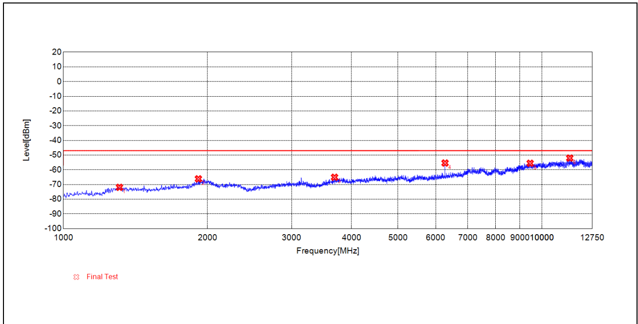
(RX_RSE_BLE_1Mbps_2480MHz_1GHz to 12.75GHz_Antenna Horizontal)
