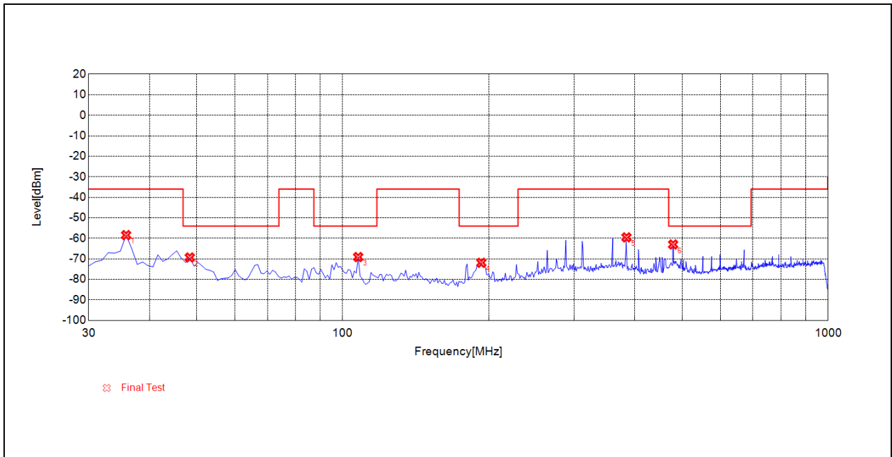
(TX_RSE_BLE_1Mbps_2402MHz_30MHz to 1GHz_Antenna Vertical)
