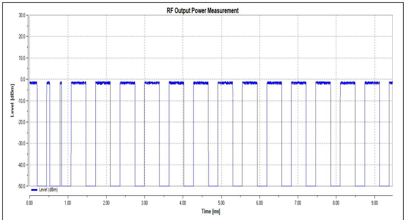
(Output Power_ BLE_1Mbps_2440MHz)
