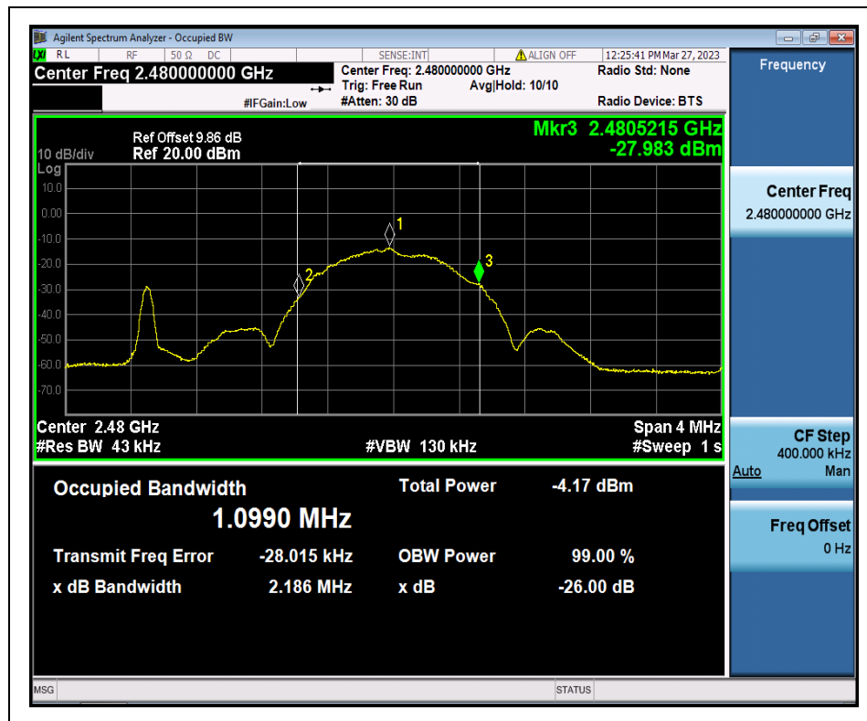
(Occupied Channel Bandwidth_BLE_1Mbps_2480MHz)
