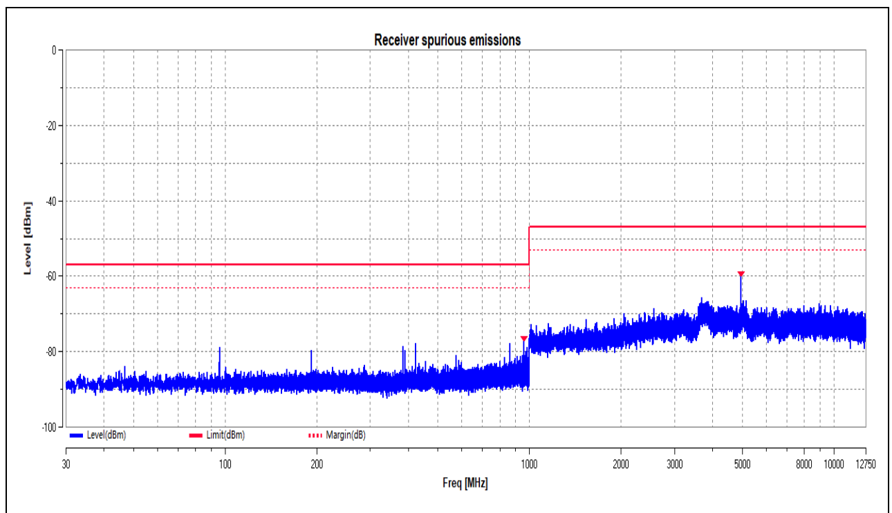
(RX_CSE_BLE_1Mbps_2480MHz_30MHz to 12.75GHz)
