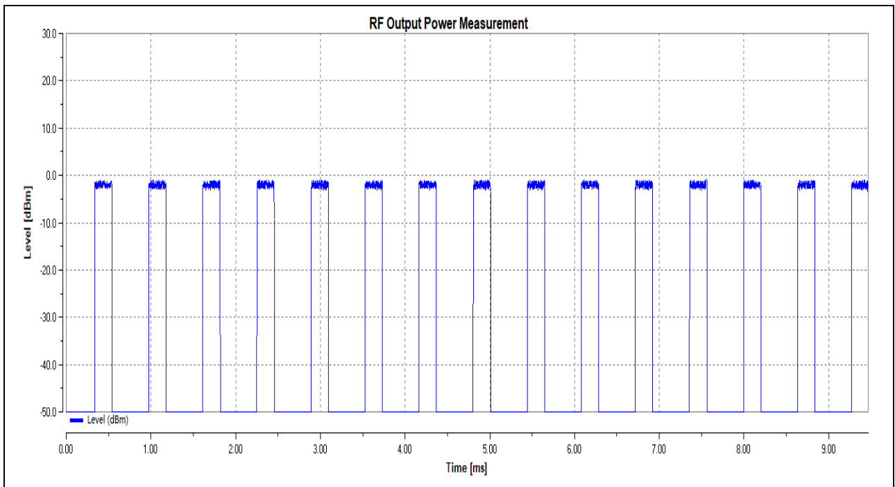
(Output Power_ BLE_2Mbps_ 2402MHz)
