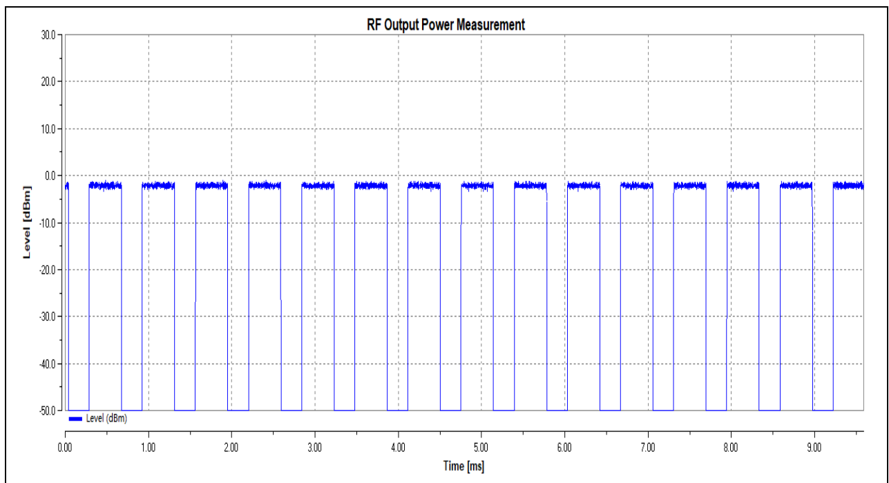
(Output Power_ BLE_1Mbps_2480MHz)
