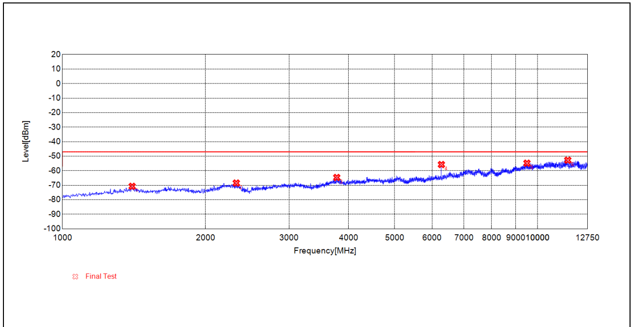
(RX_RSE_BLE_2Mbps_2402MHz_1GHz to 12.75GHz_Antenna Vertical)
