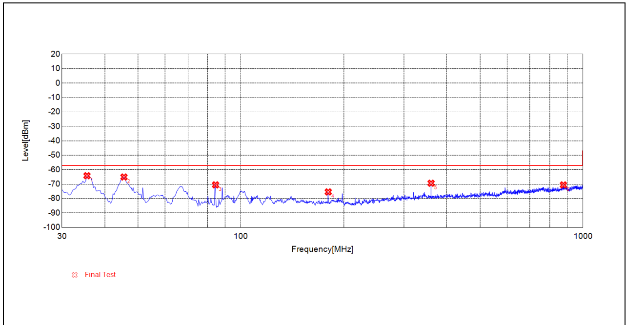
(RX_RSE_BLE_2Mbps_2402MHz_30MHz to 1GHz_Antenna Vertical)
