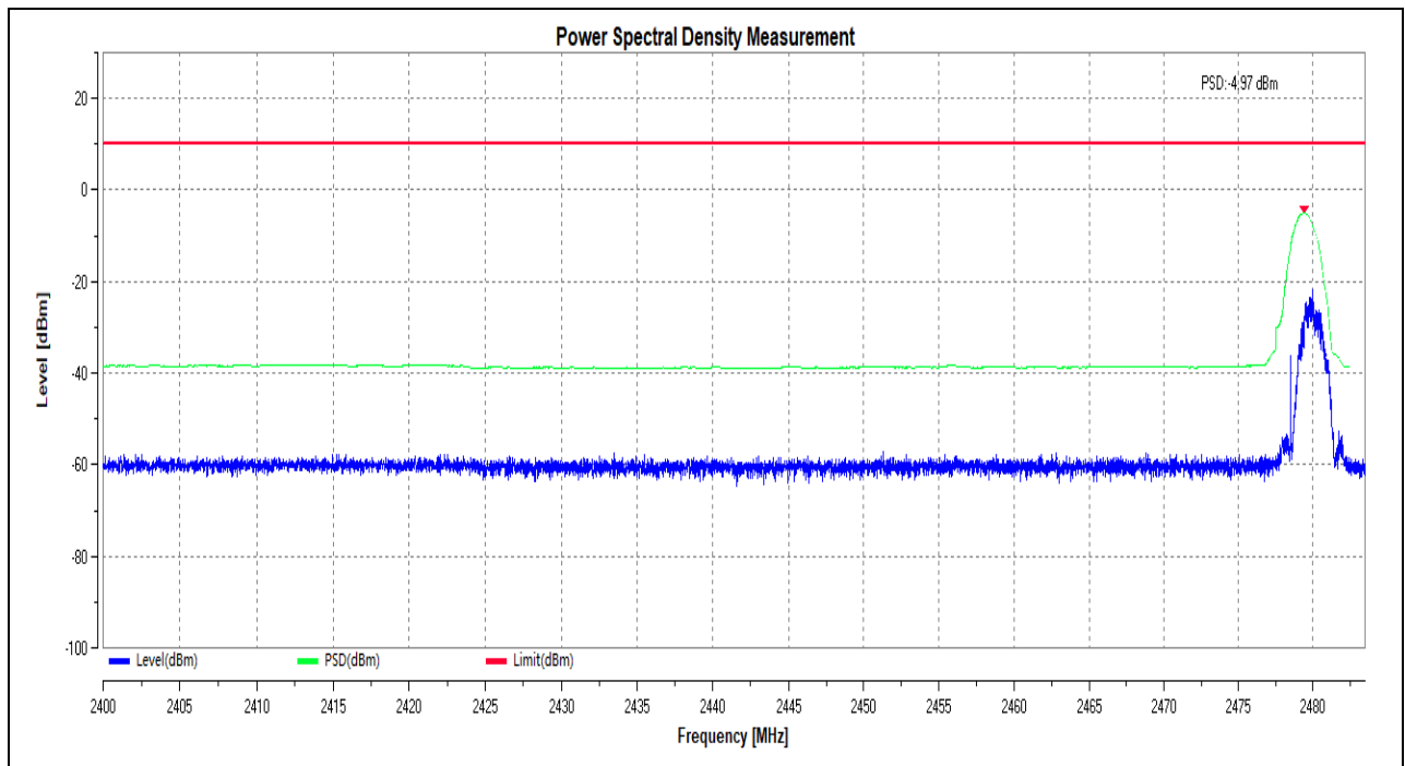
(Power Spectral Density _BLE_2Mbps_2480MHz)
