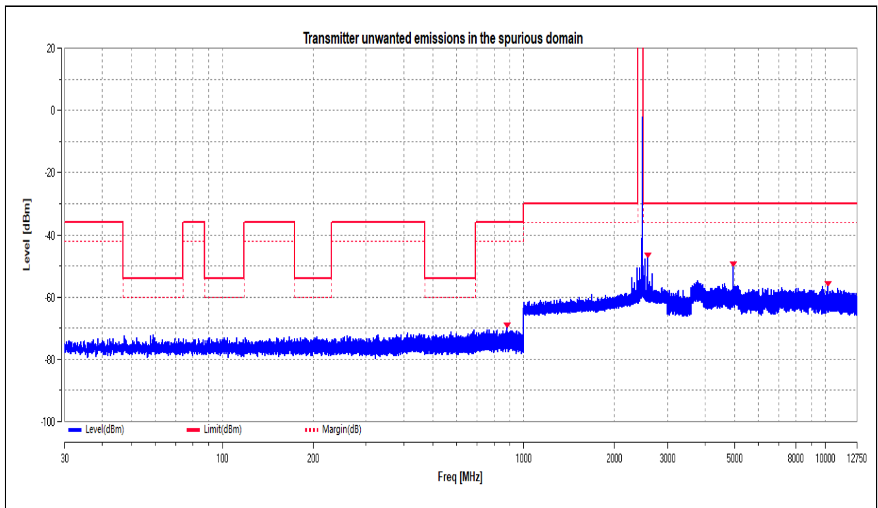
(TX_CSE_BLE_2Mbps_2480MHz_30MHz to 12.75GHz)
