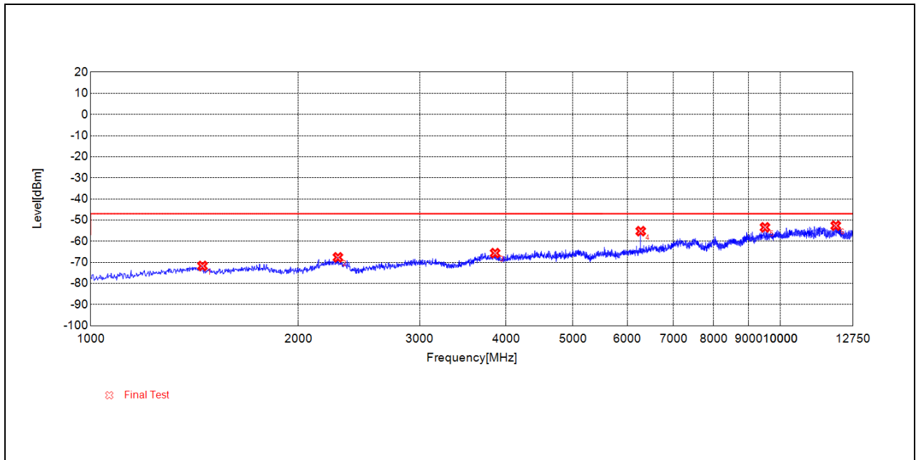
(RX_RSE_BLE_1Mbps_2480MHz_1GHz to 12.75GHz_Antenna Vertical)
