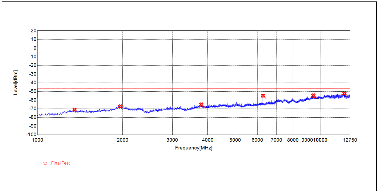
(RX_RSE_BLE_2Mbps_2480MHz_1GHz to 12.75GHz_Antenna Horizontal)
