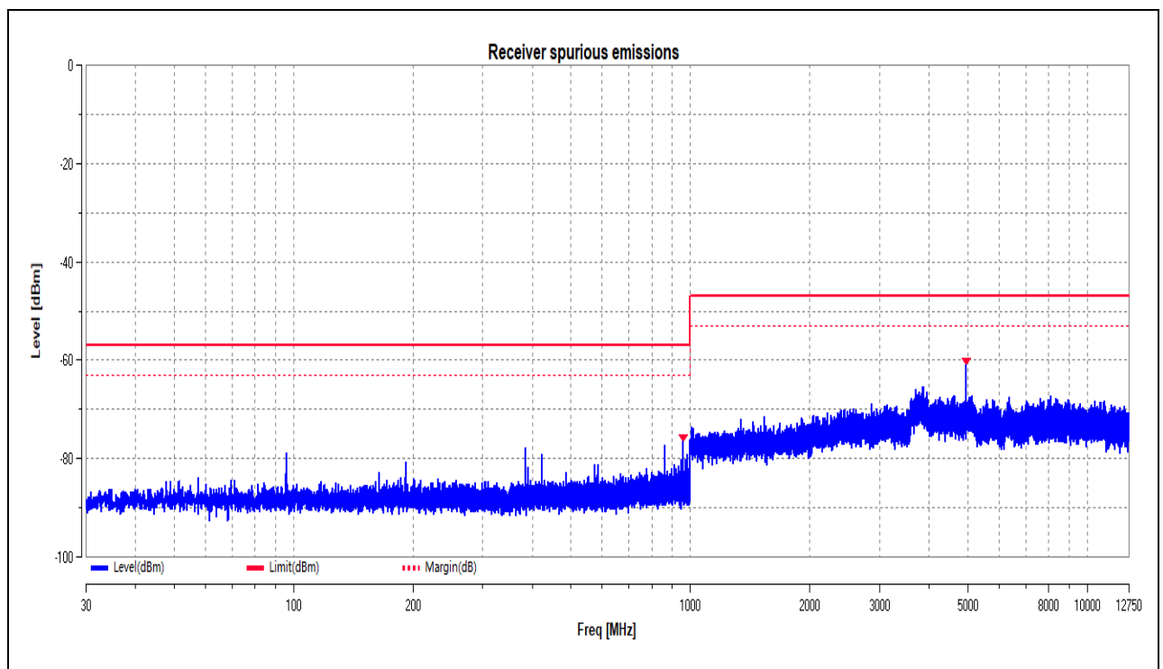
(RX_CSE_BLE_2Mbps_2480MHz_30MHz to 12.75GHz)
