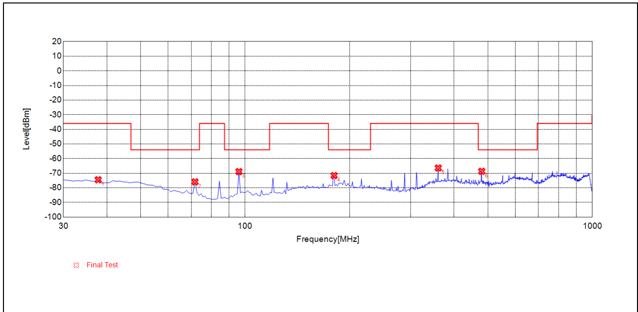
(TX_RSE_BLE_2Mbps_2480MHz_30MHz to 1GHz_Antenna Vertical)
