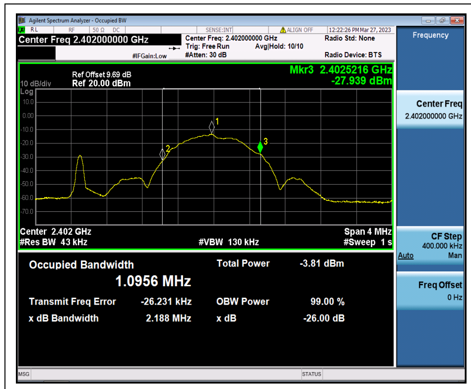
(Occupied Channel Bandwidth_BLE_1Mbps_2402MHz)
