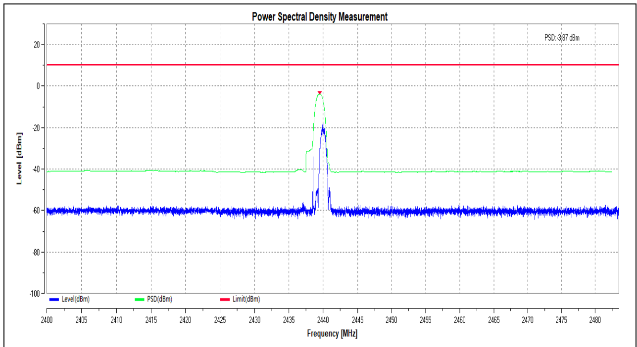
(Power Spectral Density_BLE_1Mbps_2440MHz)
