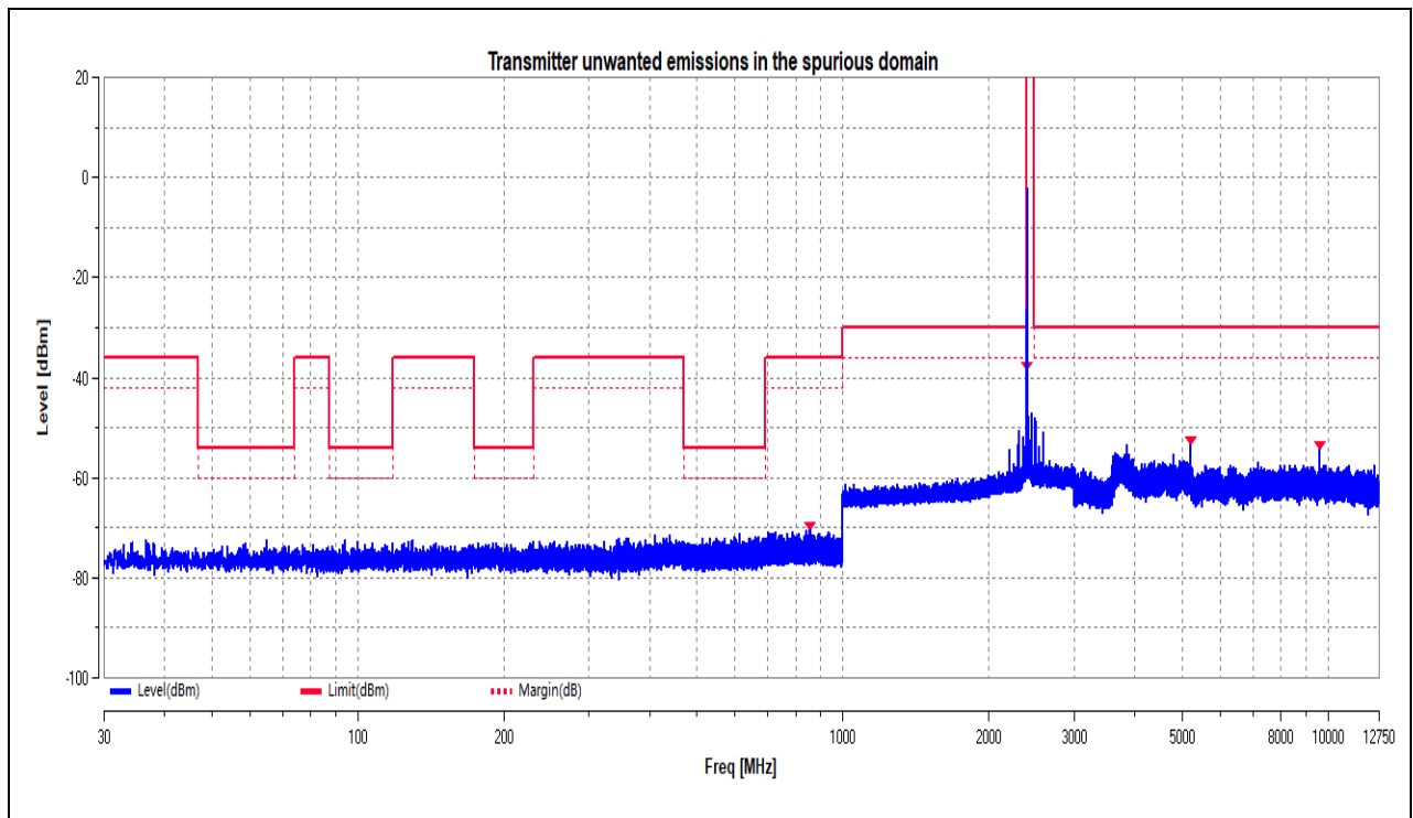
(TX_CSE_BLE_1Mbps_2402MHz_30MHz to 12.75GHz)
