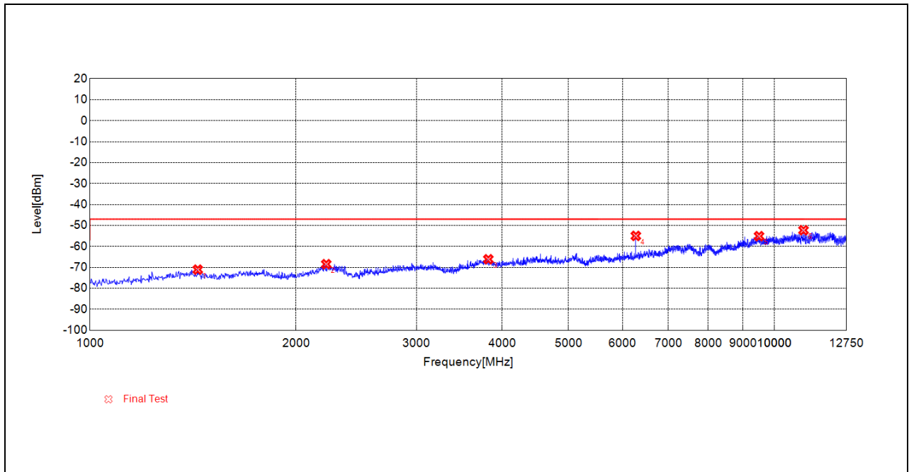
(RX_RSE_BLE_1Mbps_2402MHz_1GHz to 12.75GHz_Antenna Vertical)
