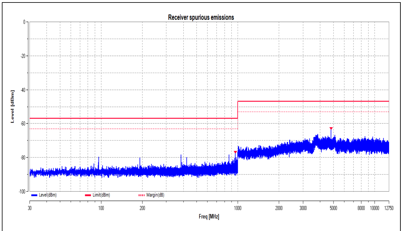
(RX_CSE_BLE_1Mbps_2402MHz_30MHz to 12.75GHz)
