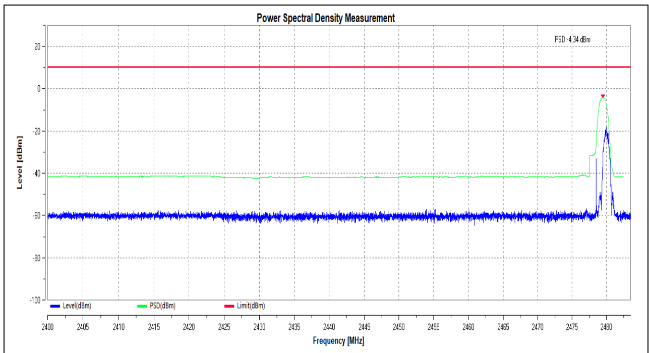
(Power Spectral Density_BLE_1Mbps_2480MHz)
