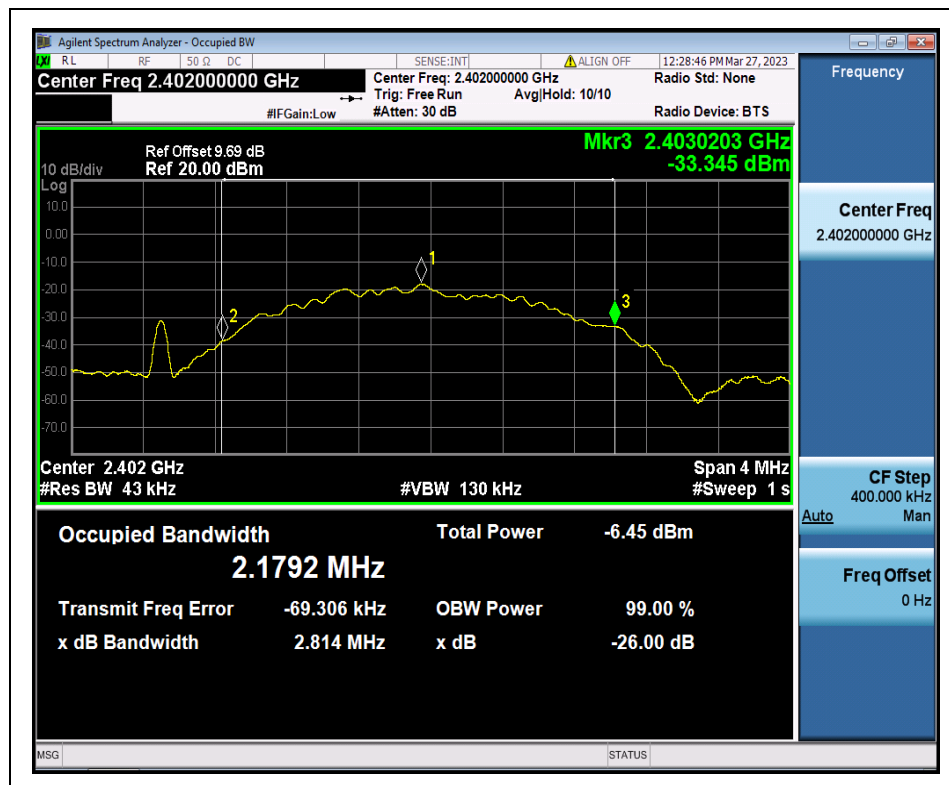
(Occupied Channel Bandwidth_BLE_2Mbps_2402MHz)
