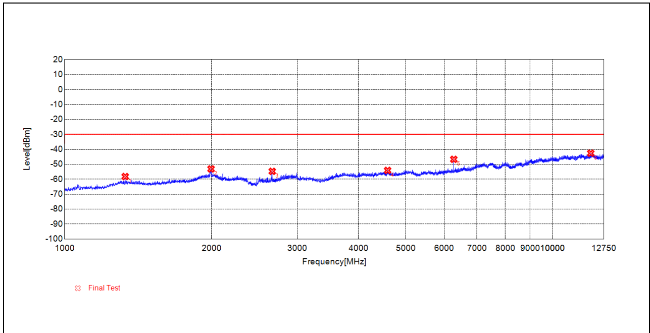
(TX_RSE_BLE_2Mbps_2480MHz_1GHz to 12.75GHz_ Antenna Horizontal)
