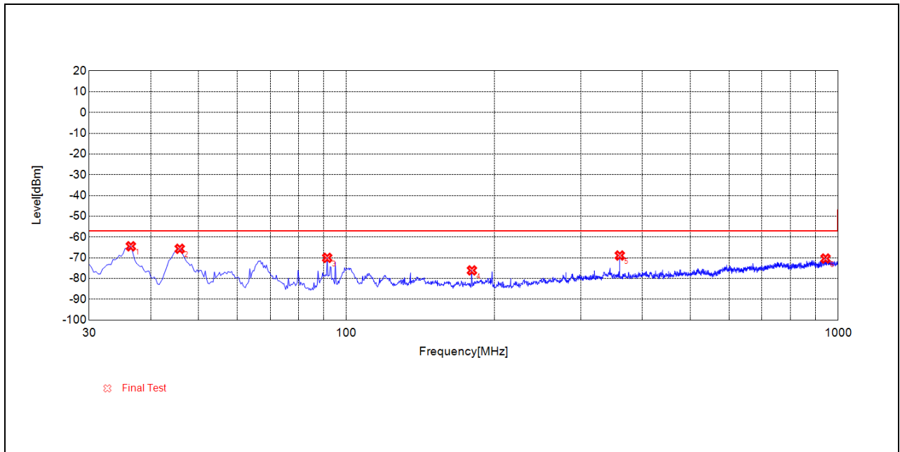
(RX_RSE_BLE_1Mbps_2480MHz_30MHz to 1GHz_Antenna Vertical)
