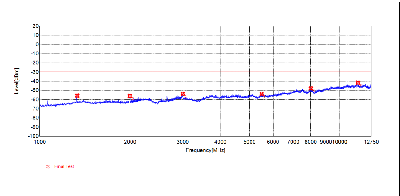
(TX_RSE_BLE_1Mbps_2480MHz_1GHz to 12.75GHz_Antenna Vertical)
