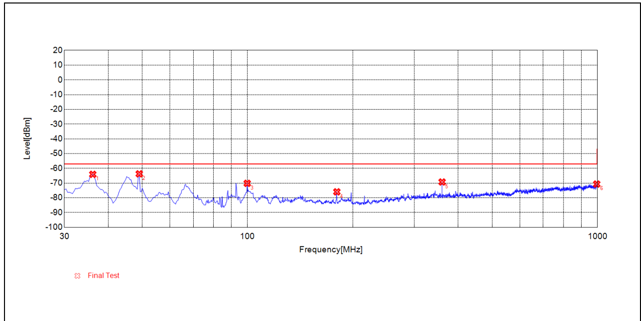
(RX_RSE_BLE_2Mbps_2480MHz_30MHz to 1GHz_Antenna Vertical)
