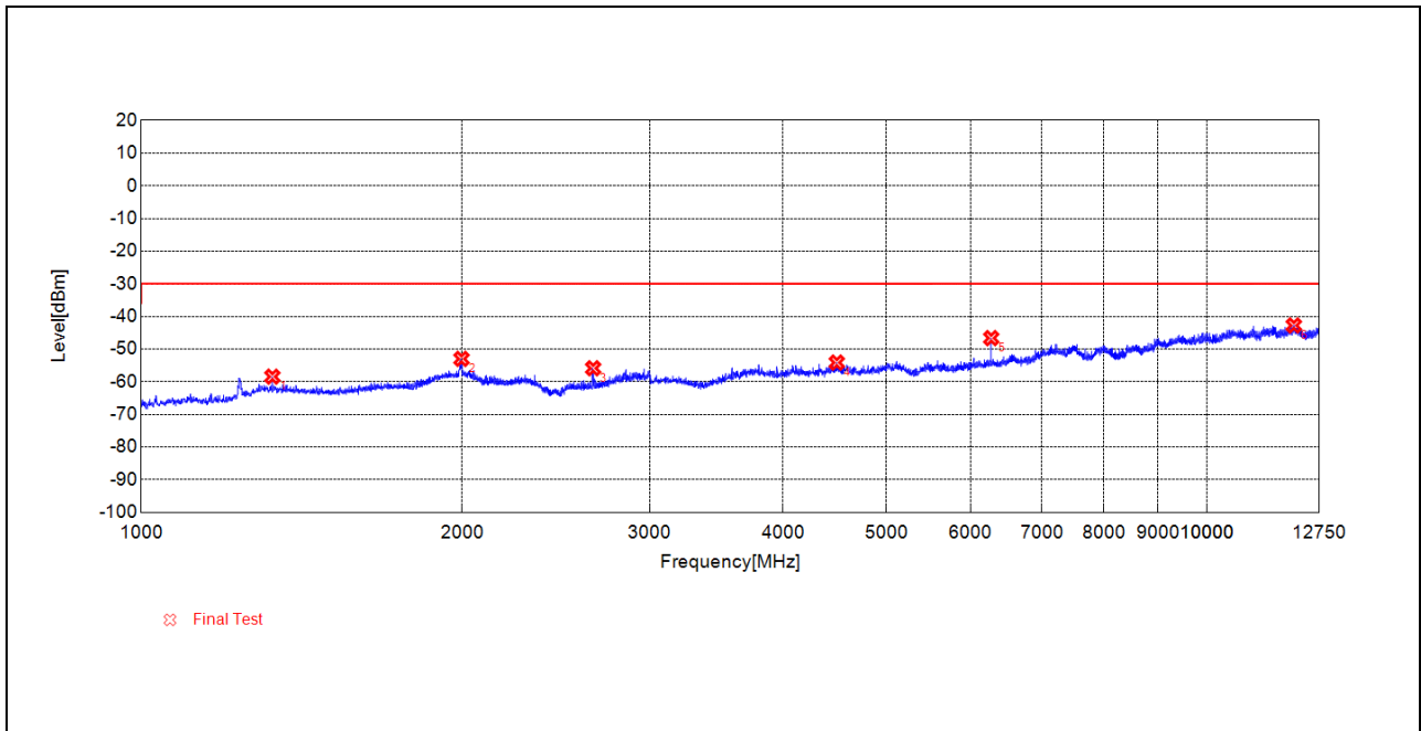
(TX_RSE_BLE_2Mbps_2402MHz_1GHz to 12.75GHz_Antenna Horizontal)
