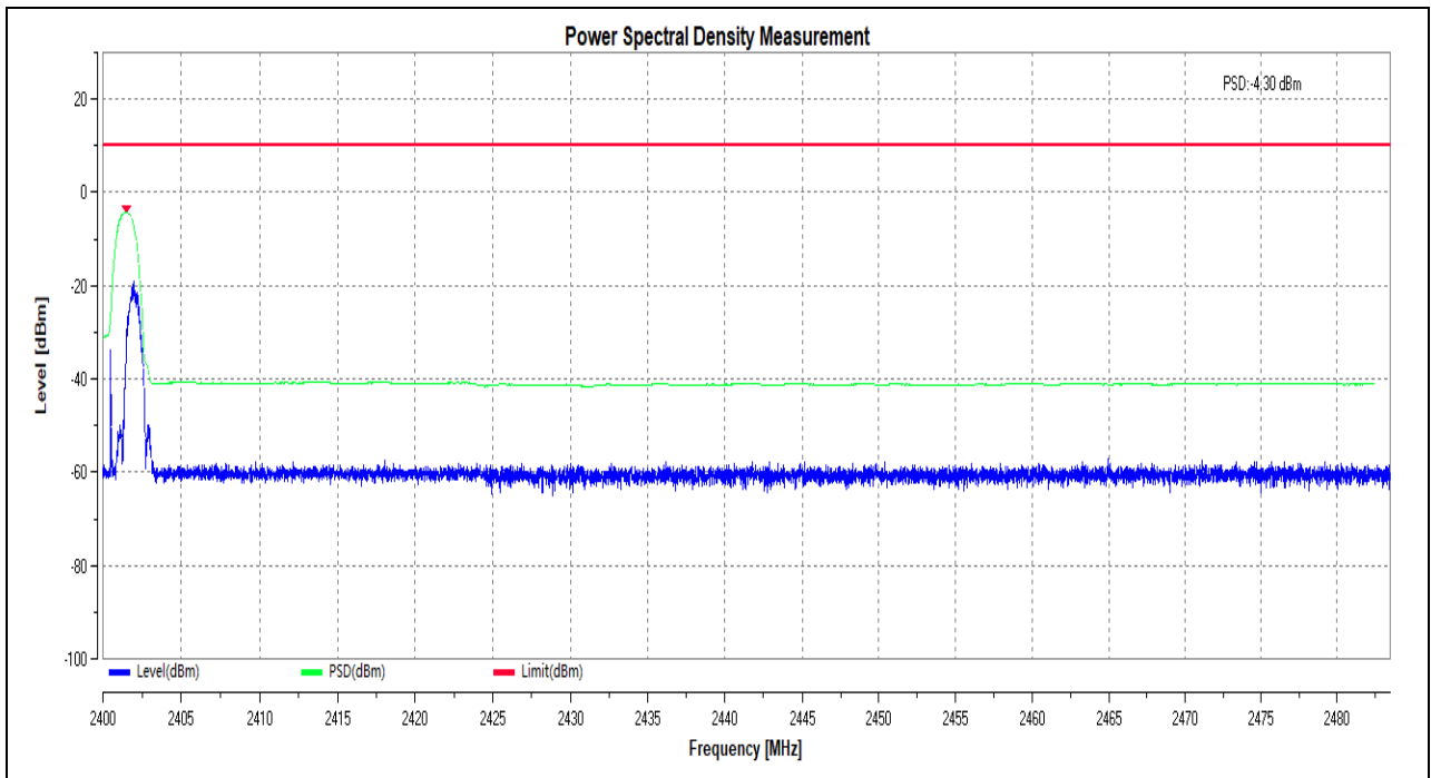
(Power Spectral Density_BLE_1Mbps_2402MHz)
