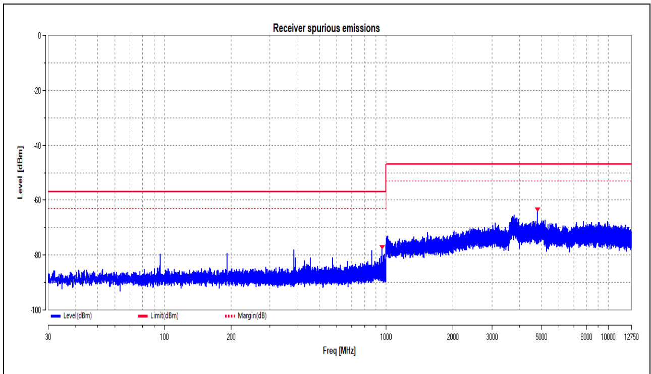
(RX_CSE_BLE_2Mbps_2402MHz_30MHz to 12.75GHz)
