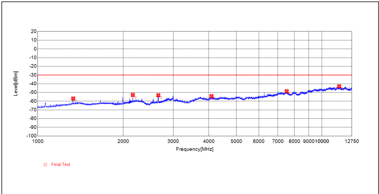
(TX_RSE_BLE_1Mbps_2402MHz_1GHz to 12.75GHz_ Antenna Vertical)
