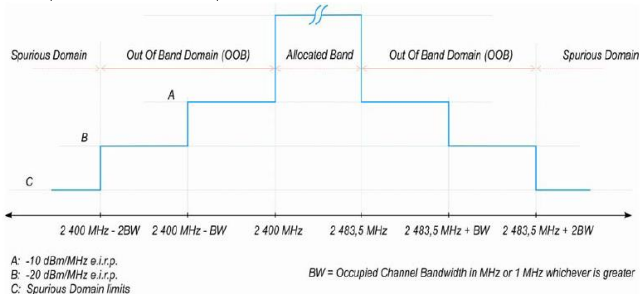
Figure 3: Transmit mask
