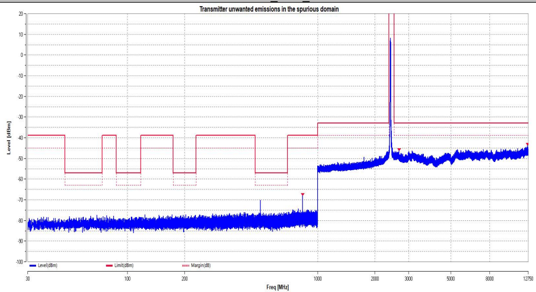
11N20MIMO Ant2 2412
