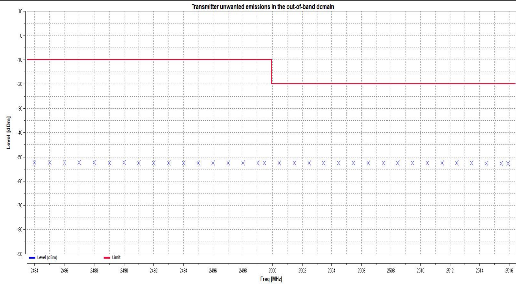
11G_Ant2_2412_2400MHz-2BW to 2400MHz
