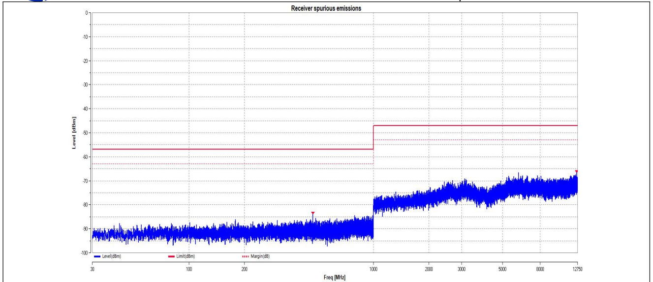
11G Ant2 2472
