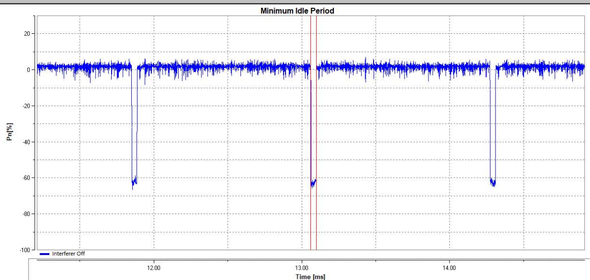
Adaptivity_Min.IdleTime_TNVN_11A_5180_Ant1
