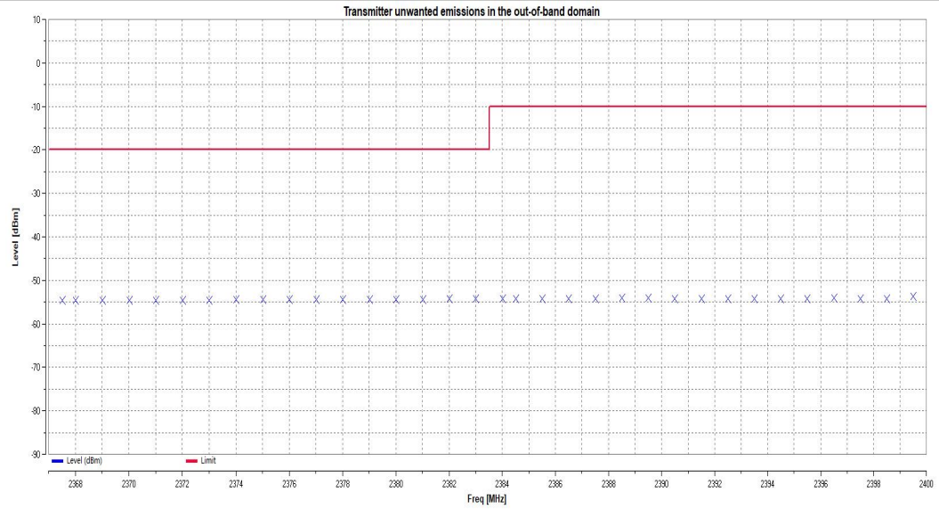
11G_Ant2_2472_2483.5MHz to 2483.5MHz+2BW
