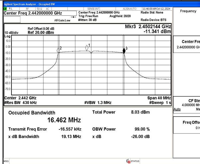
11G_Ant2_2442
