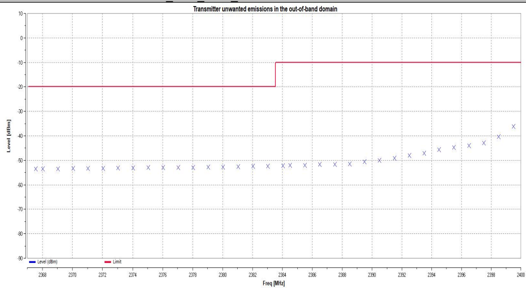
11G_Ant2_2412_2483.5MHz to 2483.5MHz+2BW
