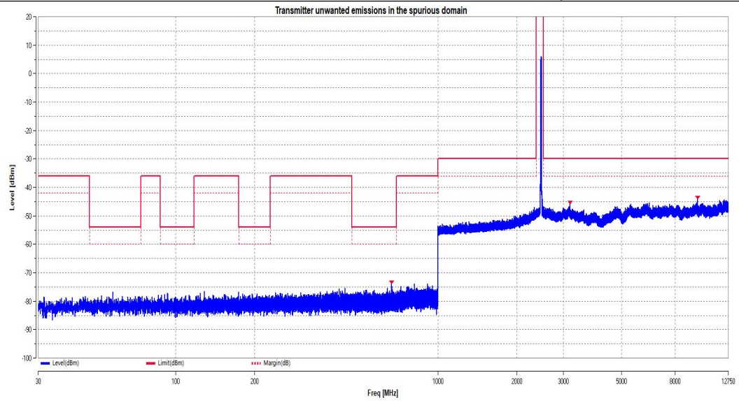
11G Ant2 2472
