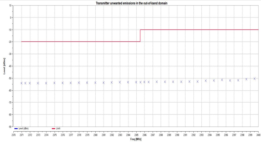
11B_Ant2_2412_2483.5MHz to 2483.5MHz+2BW
