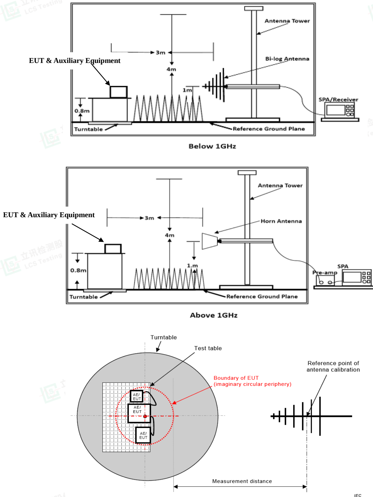
Figure C.1 – Measurement distance Test Setup for FM Receiver
