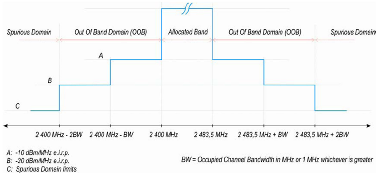
Figure 1: Transmit mask
