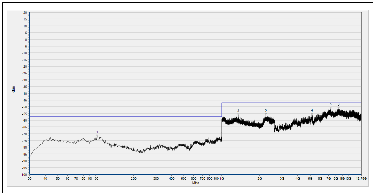
(RX_RSE_BLE_1Mbps_2402MHz_30MHz to 12.75GHz_Antenna Horizontal)
