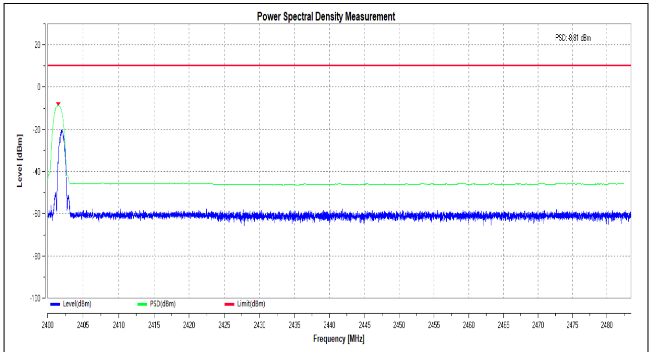
(Power Spectral Density_BLE_1Mbps_2402MHz)
