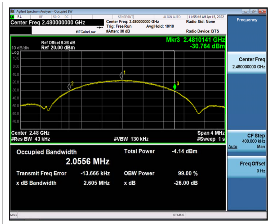
(Occupied Channel Bandwidth_BLE_2Mbps_2480MHz)
