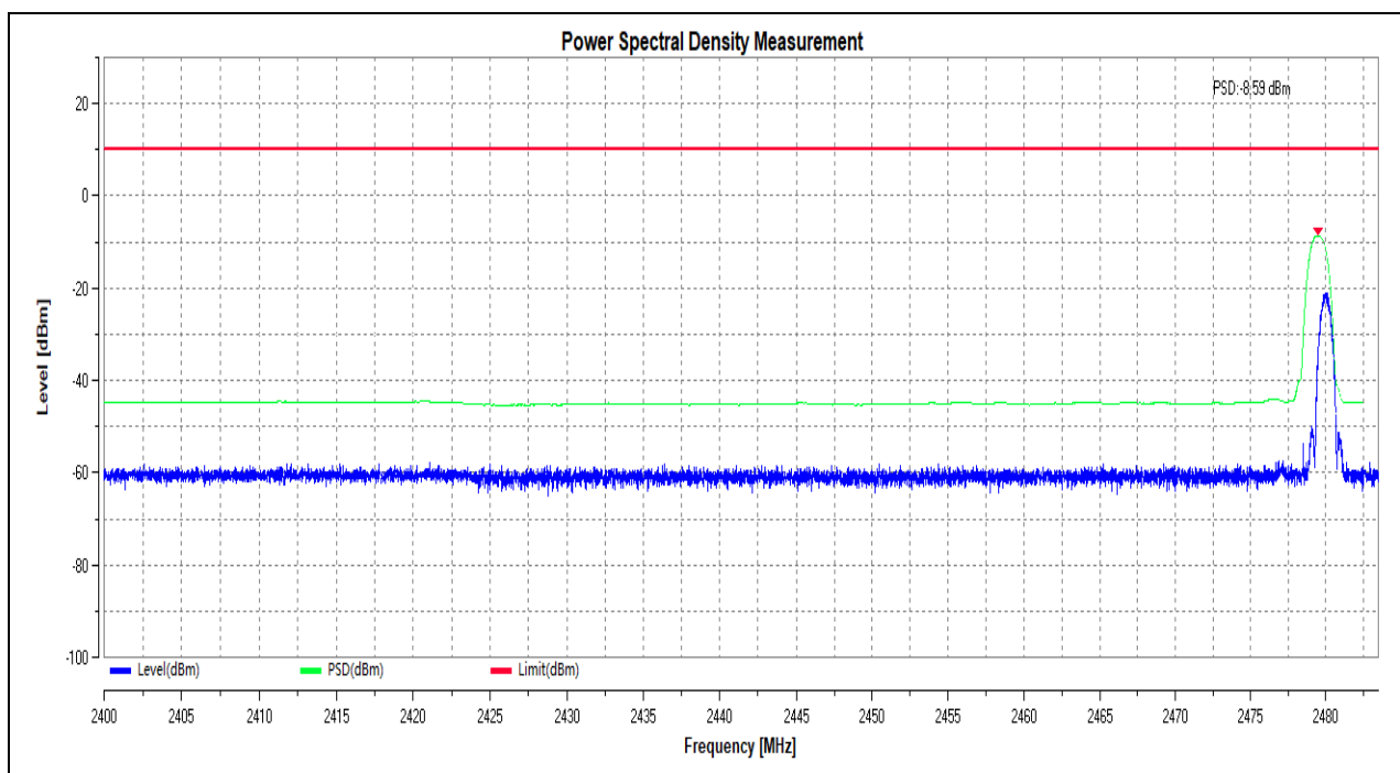
(Power Spectral Density_BLE_1Mbps_2480MHz)
