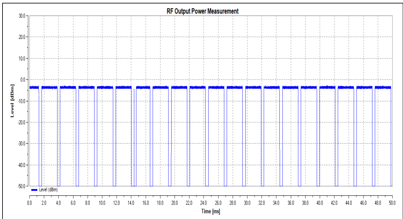
(Output Power_ BLE_1Mbps_2480MHz)
