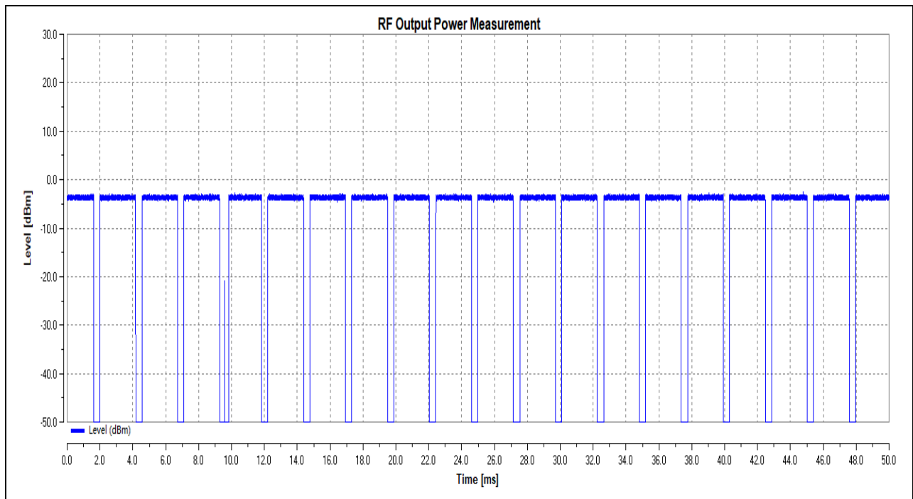
(Output Power_ BLE_1Mbps_2440MHz)
