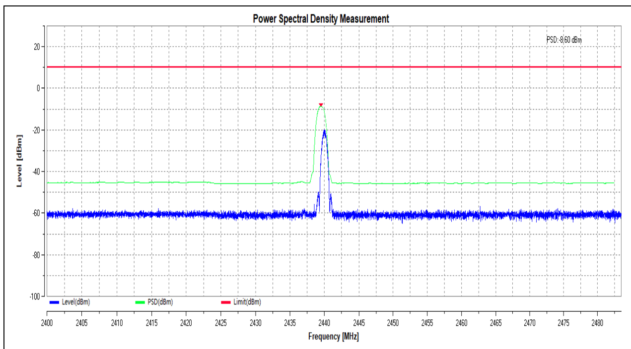
(Power Spectral Density_BLE_1Mbps_2440MHz)
