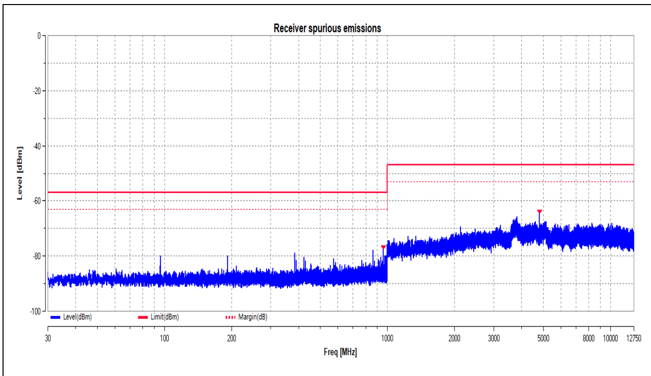
(RX_CSE_BLE_2Mbps_2402MHz_30MHz to 12.75GHz)
