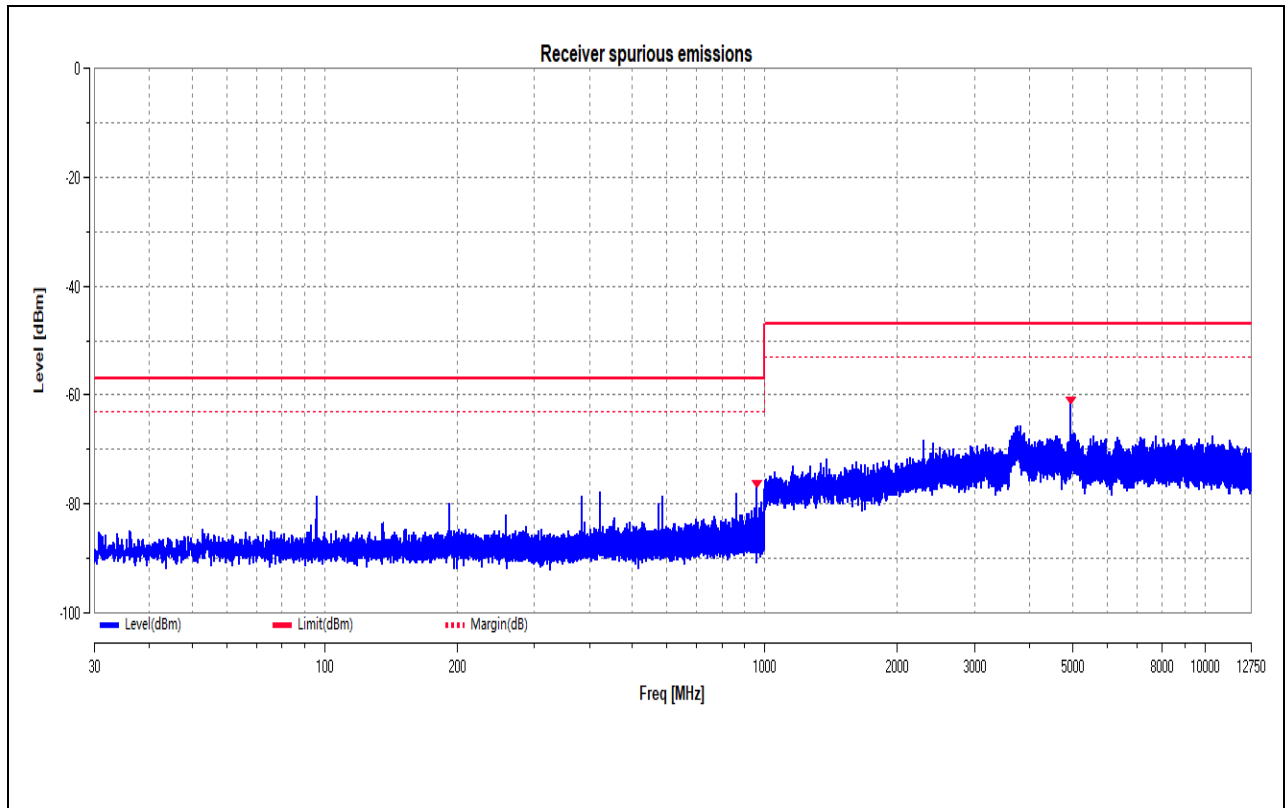
(RX_CSE_BLE_1Mbps_2480MHz_30MHz to 12.75GHz)
