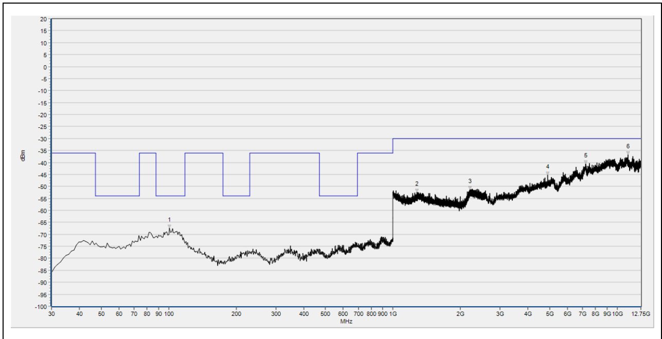
(TX_RSE_BLE_2Mbps_2402MHz_30MHz to 12.75GHz_ Antenna Vertical)
