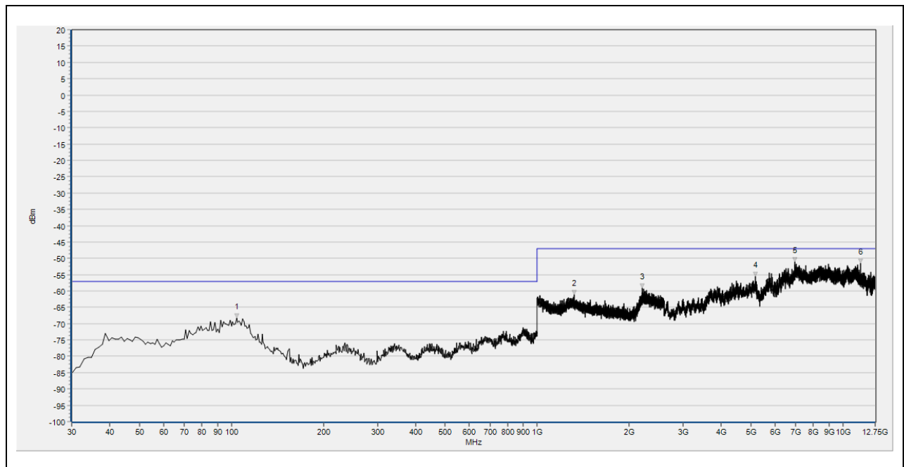
(RX_RSE_BLE_1Mbps_2402MHz_30MHz to 12.75GHz_Antenna Horizontal)
