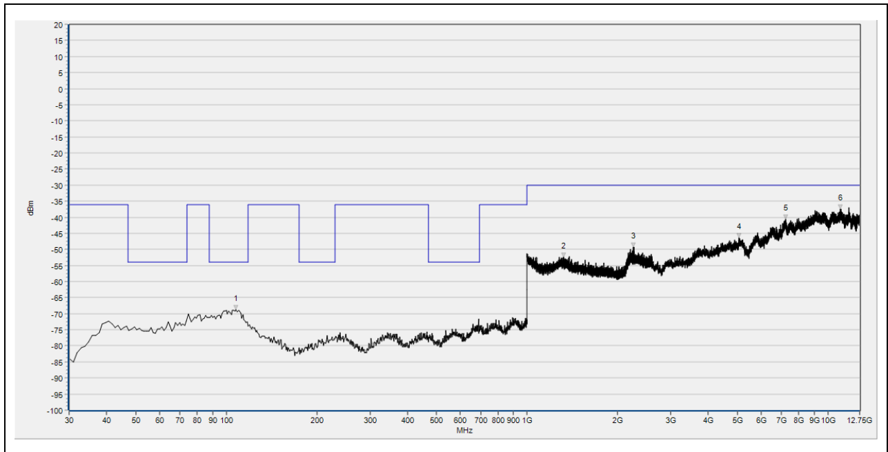
(TX_RSE_BLE_1Mbps_2480MHz_30MHz to 12.75GHz_Antenna Vertical)
