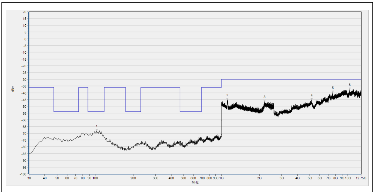
(TX_RSE_BLE_1Mbps_2402MHz_30MHz to 12.75GHz_ Antenna Horizontal)
