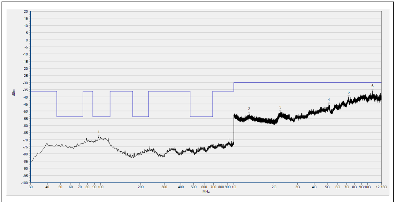
(TX_RSE_BLE_1Mbps_2402MHz_30MHz to 12.75GHz_ Antenna Vertical)
