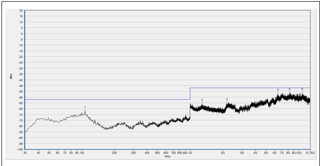
(RX_RSE_BLE_1Mbps_2402MHz_30MHz to 12.75GHz_Antenna Vertical)
