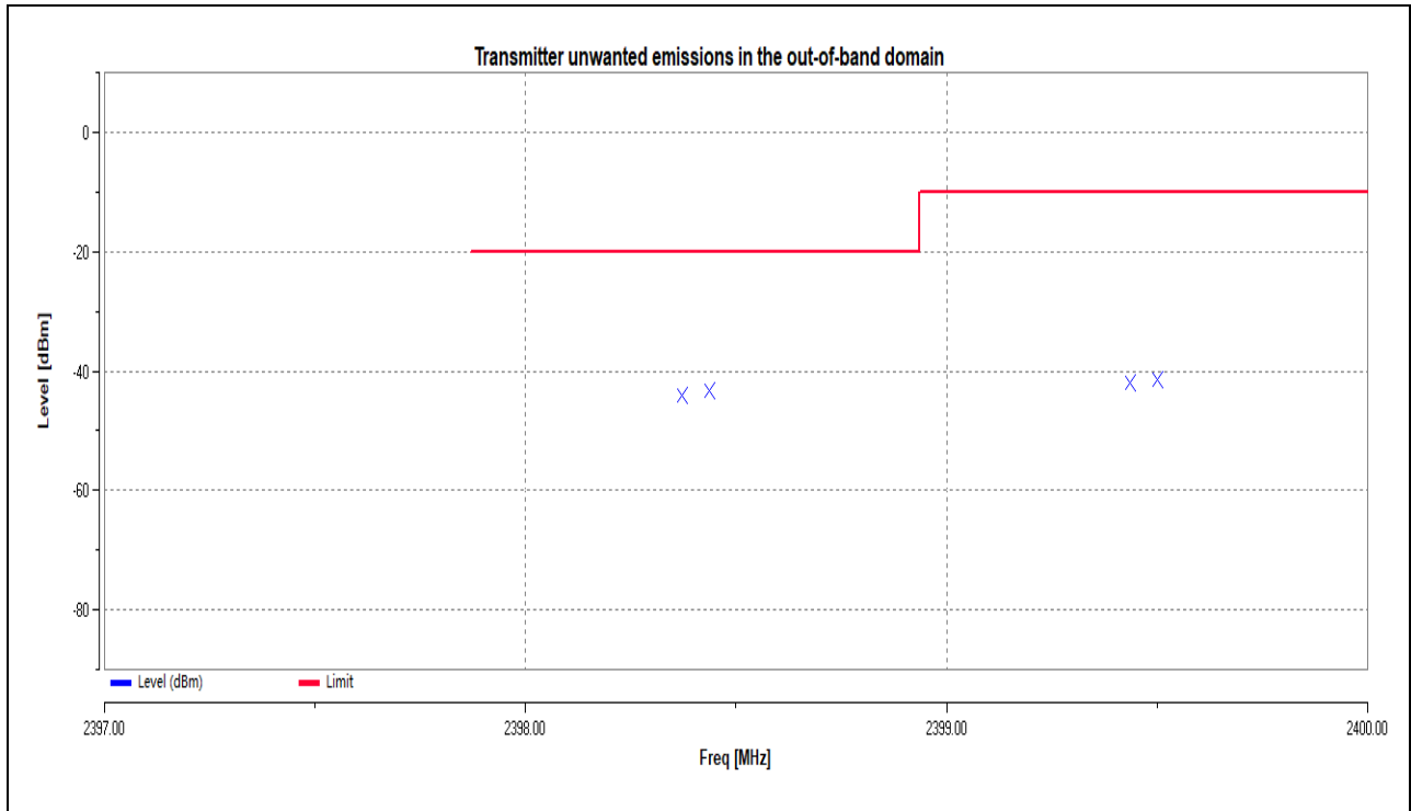
(OOB_BLE_1Mbps_2402MHz)
