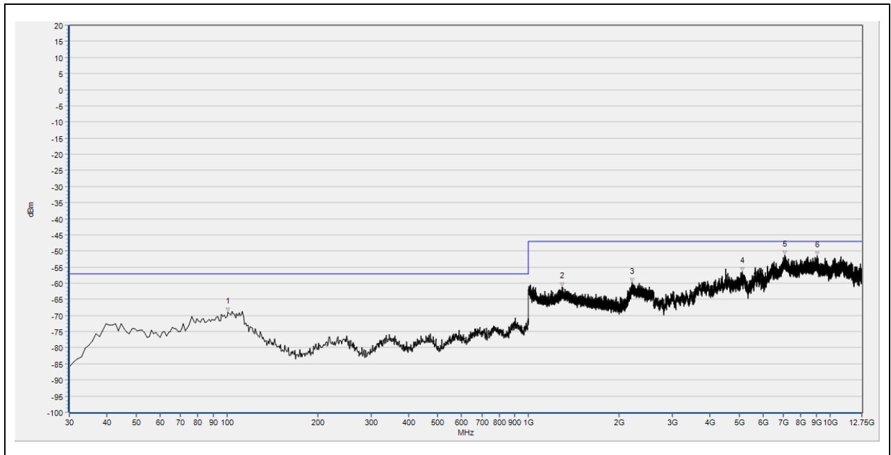
(RX_RSE_BLE_2Mbps_2480MHz_30MHz to 12.75GHz_Antenna Vertical)
