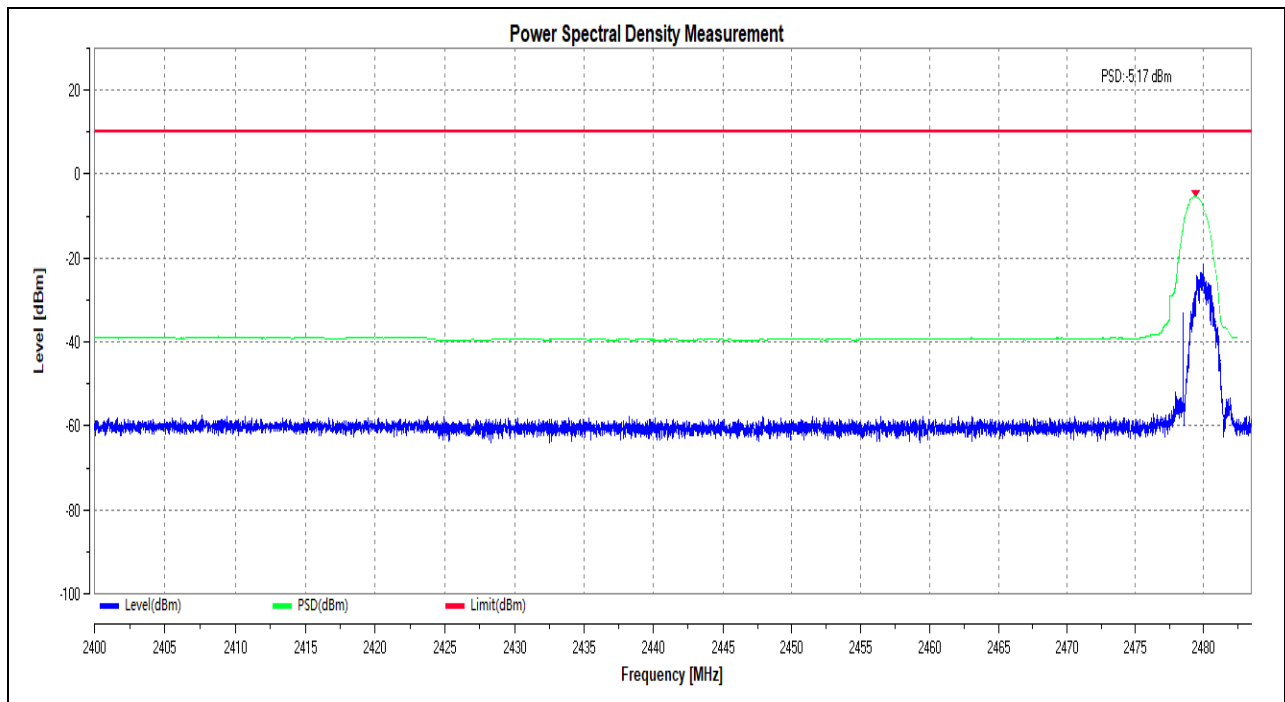
(Power Spectral Density _BLE_2Mbps_2480MHz)
