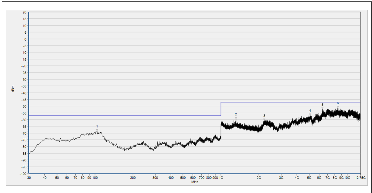
(RX_RSE_BLE_2Mbps_2402MHz_30MHz to 12.75GHz_Antenna Vertical)
