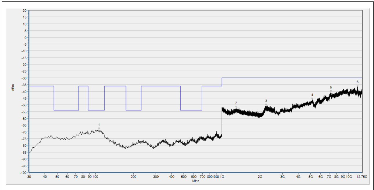
(TX_RSE_BLE_2Mbps_2480MHz_30MHz to 12.75GHz_Antenna Vertical)
