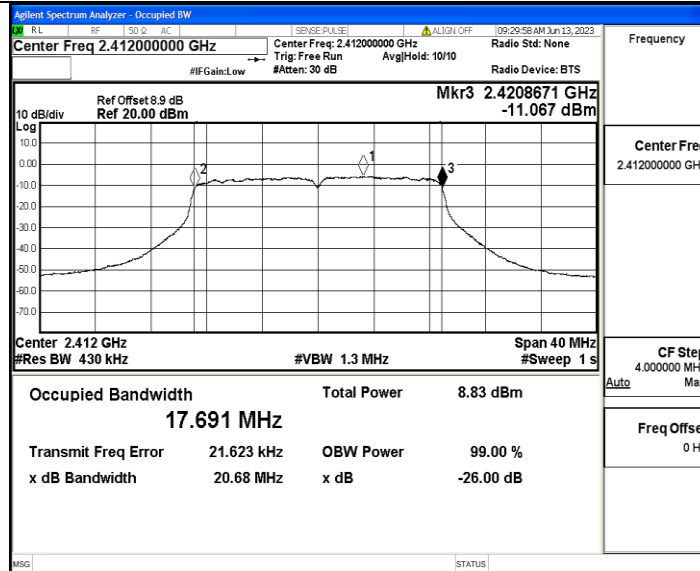
11N20SISO_Ant1_2442
