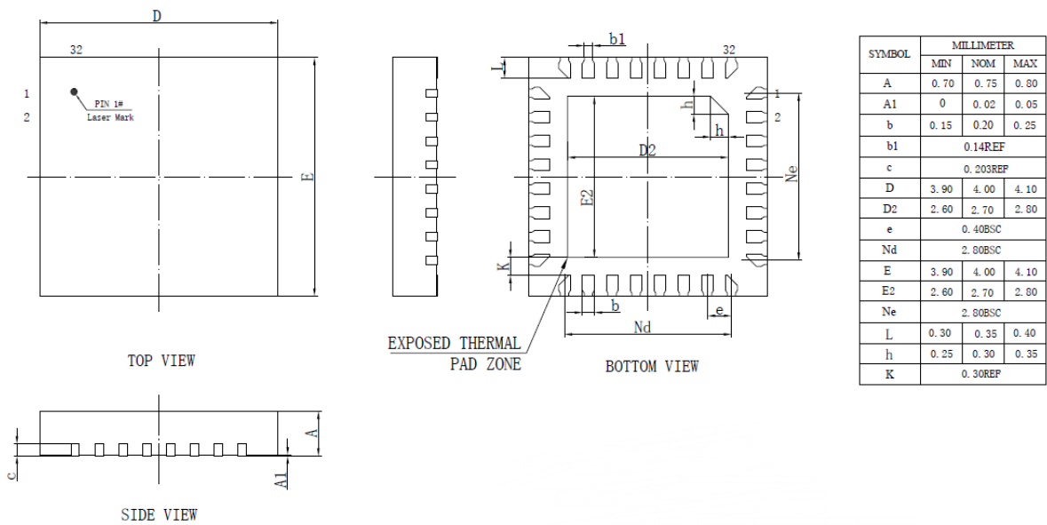
Figure 3-1. AC6966B_QFN32 Package
