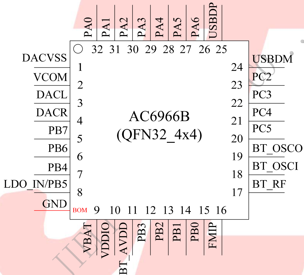
Figure 1-1 AC6966B_QFN32 Package Diagram
